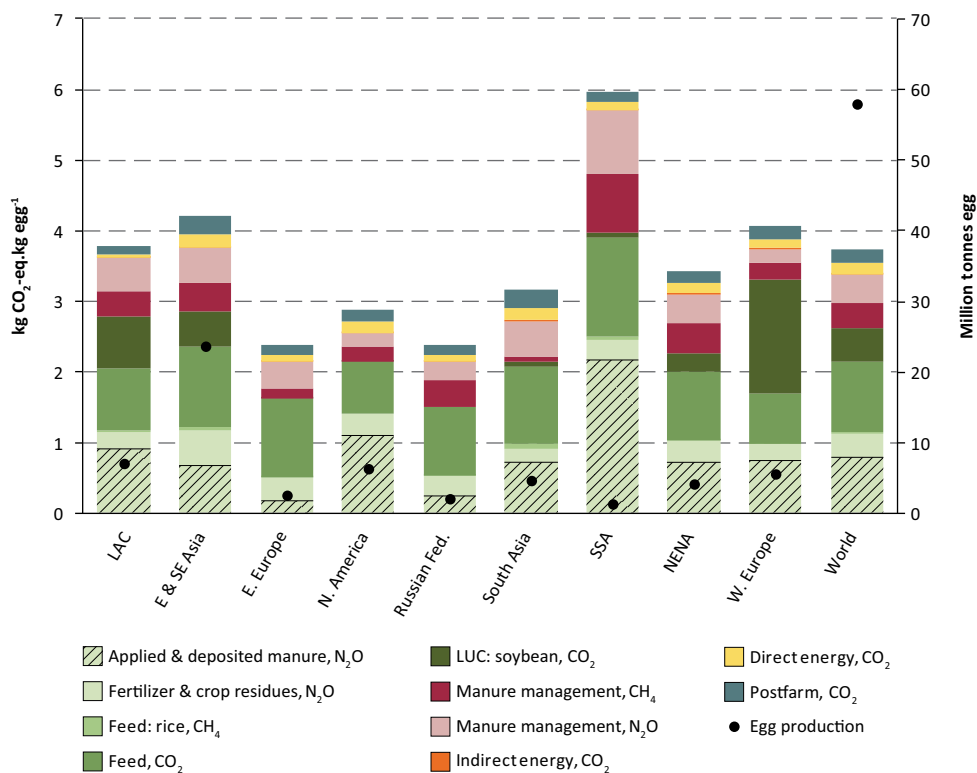
FIGURE 22. Regional variation in chicken egg production and GHG emission intensities*
