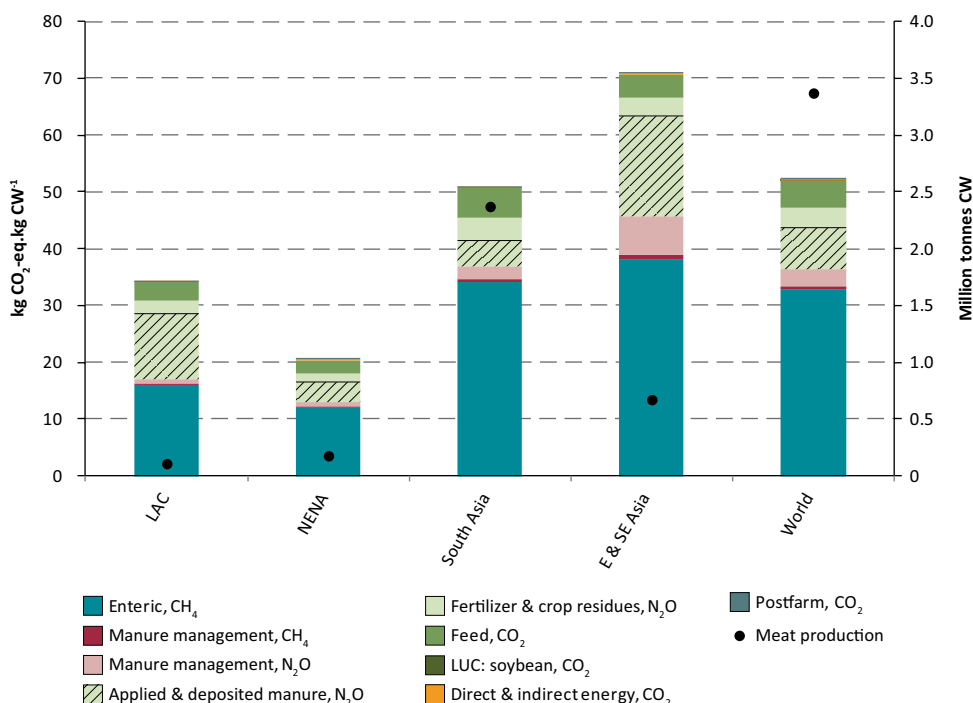
FIGURE 13. Regional variation in buffalo meat production and GHG emission intensities*
