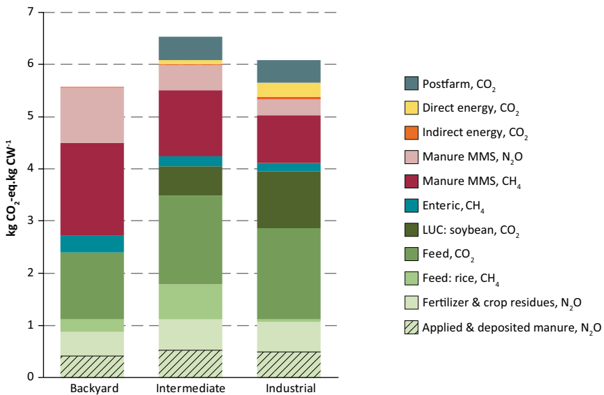
FIGURE 24. Global emission intensity from pig supply chains, by main production systems
