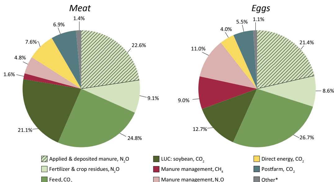
FIGURE 20. Global emissions from chicken meat and egg supply chains, by category of emissions
